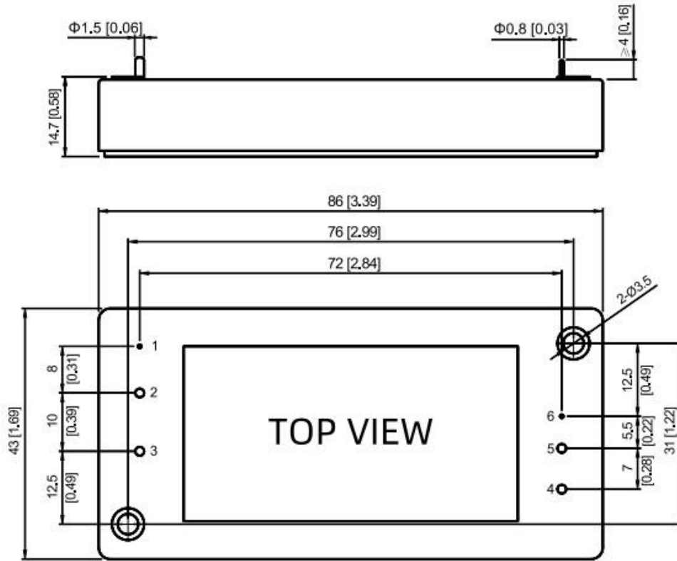
TOP VIEW
